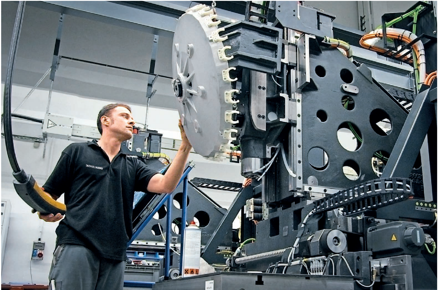
Assembling a tool changer: Dirk Ziegler, assembly fitter at DECKEL MAHO Seebach GmbH, assembles the tool changer of a MILLTAP 700.
